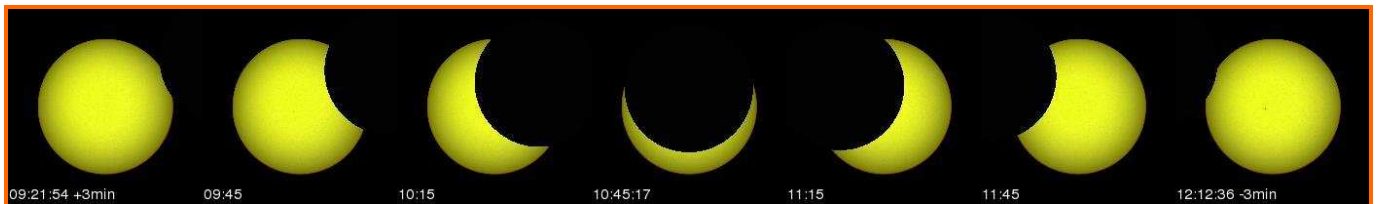
WHAT YOU WILL SEE OF THE ECLIPSE IN VILNIUS – 76.9%
